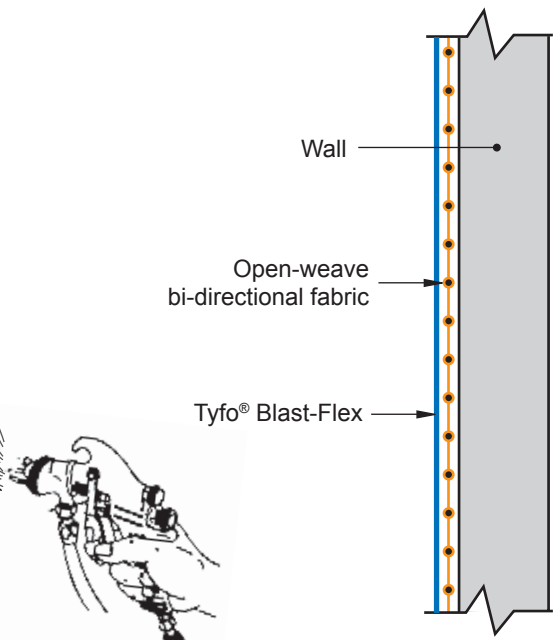
Wall Section
